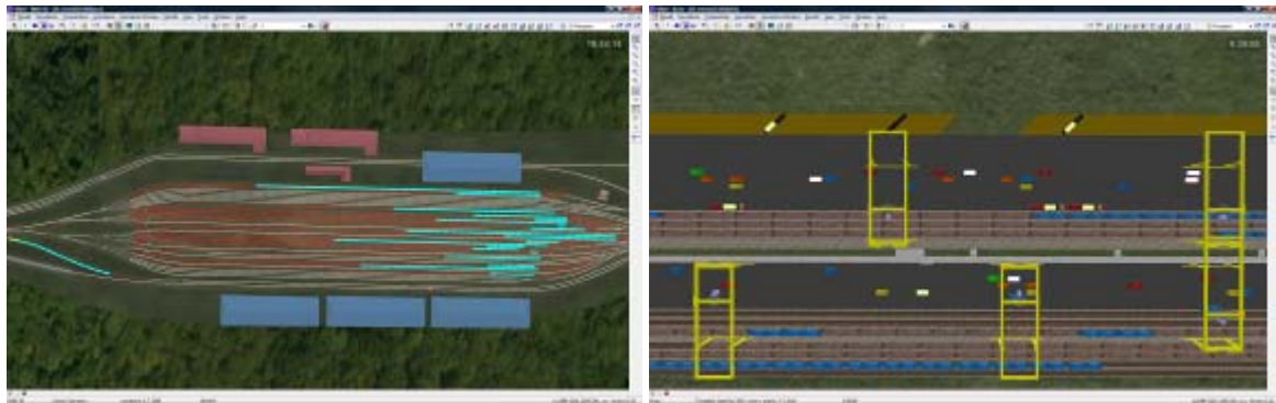
Figure 7-1 - VILLON - 3D infrastructure modelling
