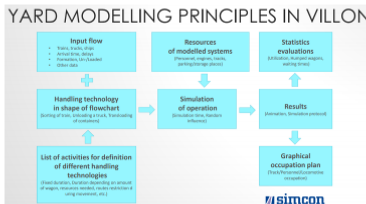
Figure 7-3 - Villon's yard modelling principles
