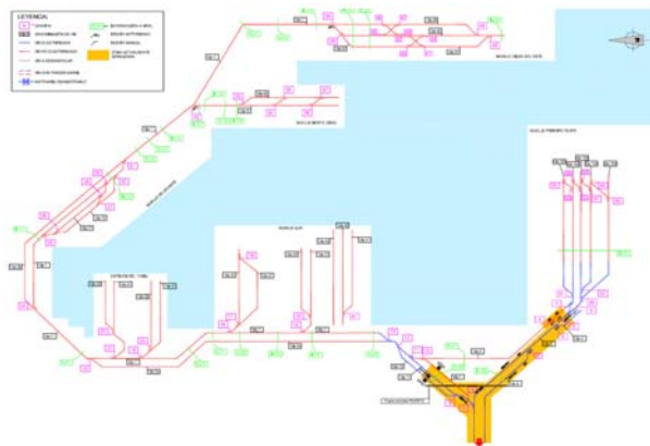
Figure 5-3 - Example of a layout of an intermodal maritime rail network (Valencia)
